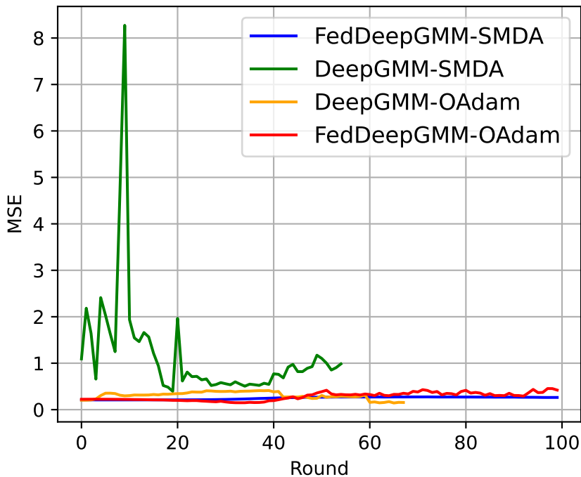
Comparison of MSE Over Rounds
